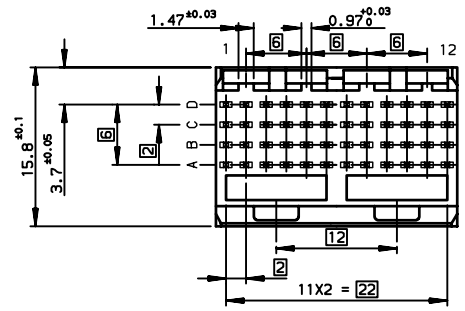
LAYOUT FOR P.C.B (PER 12mm LENGTH)
