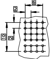
LAYOUT FOR P.C.B (PER 12mm LENGTH)
