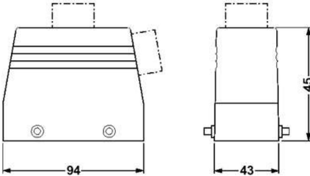
Dimensioned drawing
