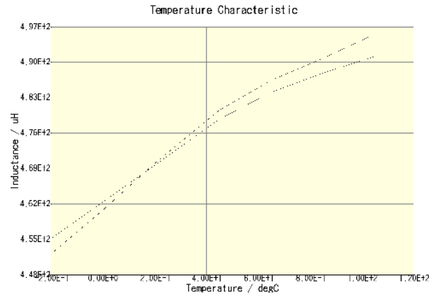
CLF7045T-471M-CA(DC = 0A)
