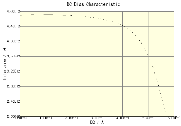
CLF7045T-471M-CA(Amb. Temp. = 20degc)
