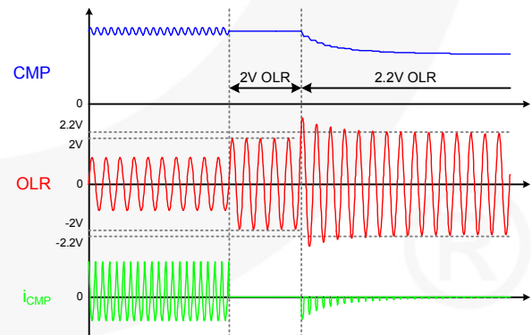
Figure 48. Open-Lamp Regulation in Normal Mode
