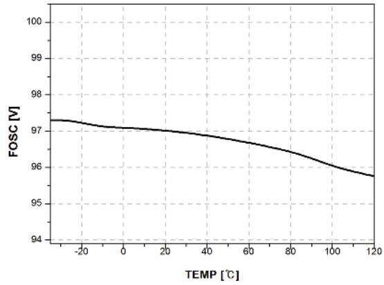
Figure 10. Oscillation Frequency vs. Temp.
