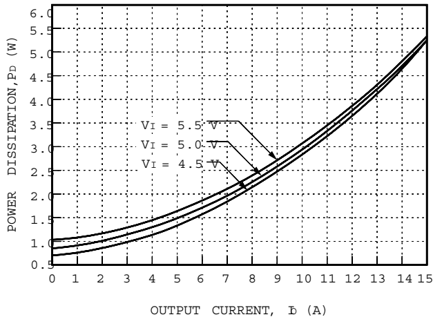
Figure 43. NH050M-L Typical Power Dissipation vs. Output Current, T_A = 25^\circ\text{C}
