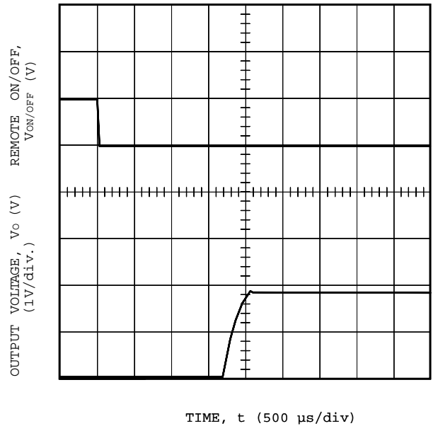
Figure 28. NH050S1R8-L Typical Start-Up from Remote On/Off, V i = 5 V, I o = 15 A
