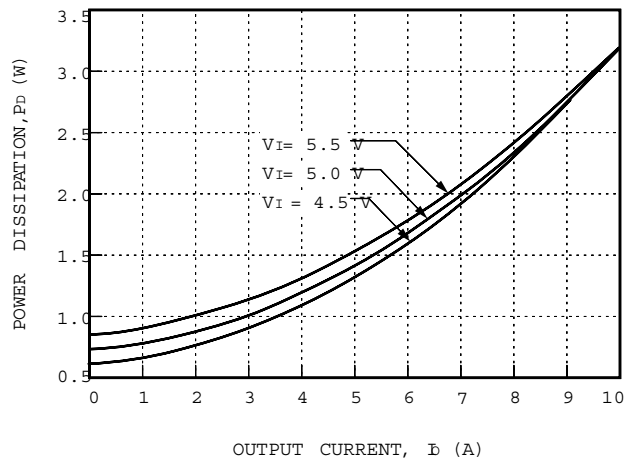
Figure 44. NH033S1R8-L Typical Power Dissipation vs. Output Current, T_A = 25^\circ\text{C}
