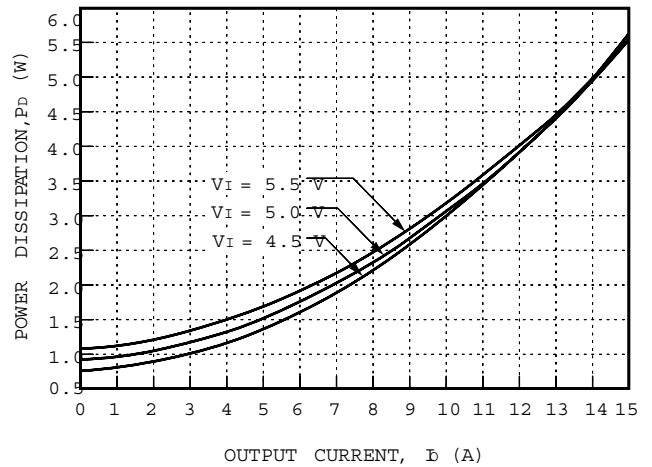
Figure 45. NH050S1R8-L Typical Power Dissipation vs. Output Current, T_A = 25^\circ\text{C}
