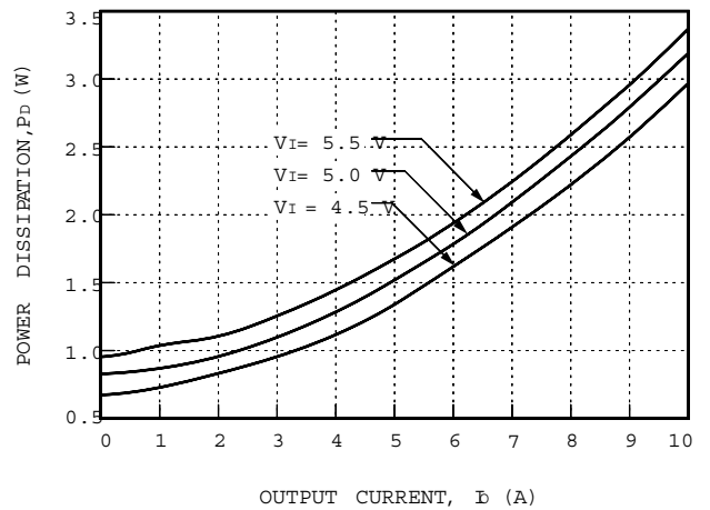
Figure 46. NH033G-L Typical Power Dissipation vs. Output Current, T_A = 25^\circ\text{C}
