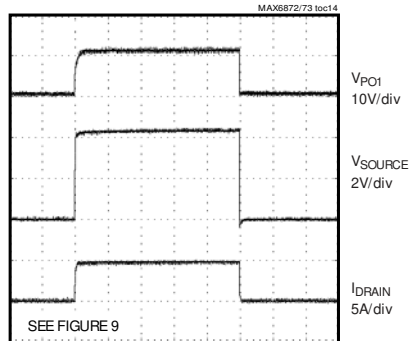
FET (IRF7811W) TURN-ON WITH CHARGE PUMP
