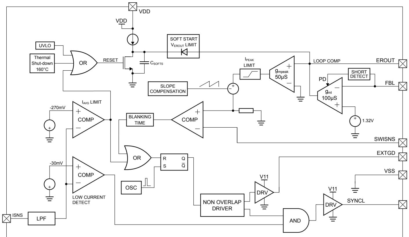
Figure 2.5. Si34071 DC-DC Converter Block Diagram
