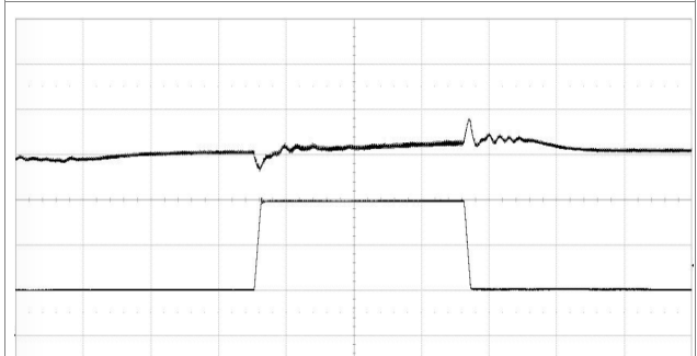
Output voltage response to load current Step-change (10-30-10 A) at: T_{P1} = +25^\circ C , V_I = 12 V , V_O = 1.0 V , di/dt = 2 A/\mu s , f_{sw} = 320 kHz , C_O = 4000 \mu F Top trace: output voltage (100 mV/div.). Bottom trace: load current (10 A/div.). Time scale: (0.1 ms/div.).
