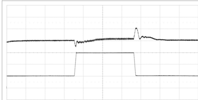
Output voltage response to load current Step-change (10-30-10 A) at: T_{P1} = +25^\circ C , V_I = 12 V , V_O = 1.0 V , di/dt = 2 A/\mu s , f_{sw} = 320 kHz , C_O = 4000 \mu F Top trace: output voltage (200 mV/div.). Bottom trace: load current (10 A/div.). Time scale: (0.1 ms/div.).
