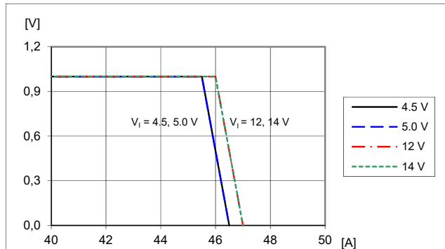
Current Limit Characteristics, V_O = 1.0\text{ V}
