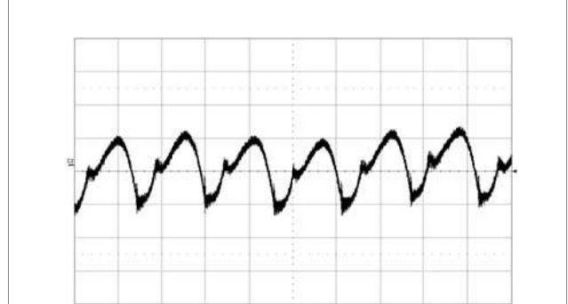
Output voltage ripple at: T_{P1} = +25\text{ }^\circ\text{C} , Trace: output voltage (10 mV/div.). V_I = 12\text{ V} , C_O = 470\text{ }\mu\text{F}/10\text{ m}\Omega Time scale: (2 \mu\text{s}/\text{div.} ). I_O = 40\text{ A} 20 MHz bandwidth
