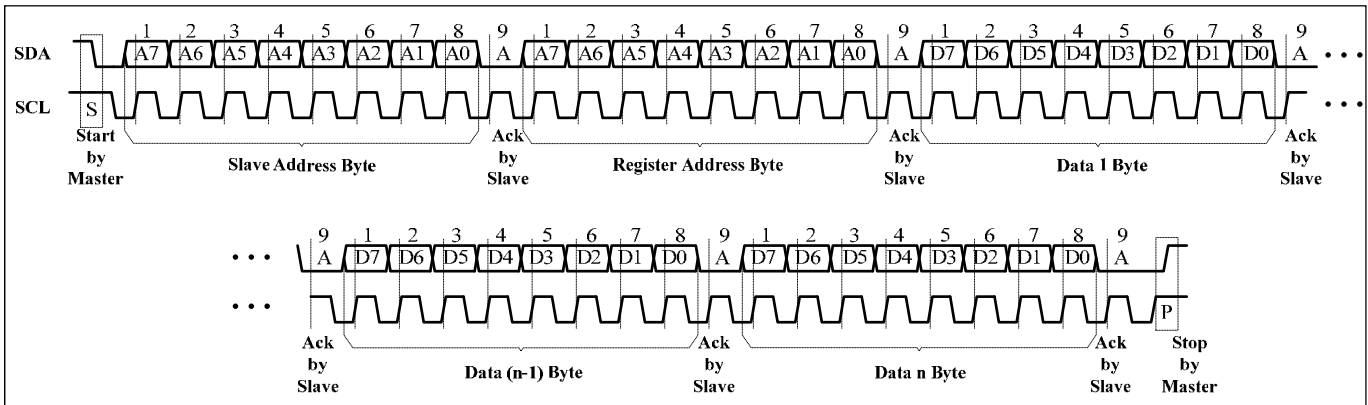
Figure 7 I2C Writing to IS31FL3716 (Automatic Address Increment)
