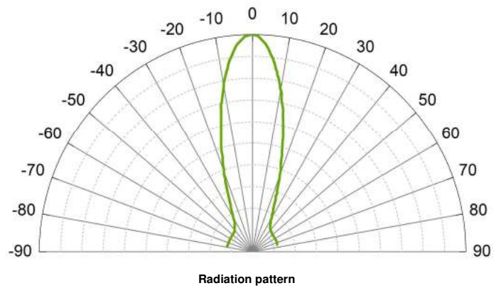
Radiation pattern
