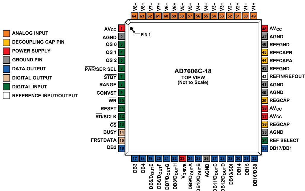
Figure 8. Pin Configuration
