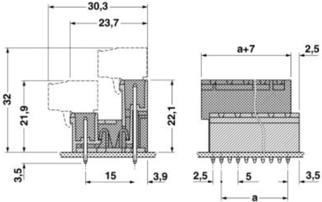
Dimensioned drawing
