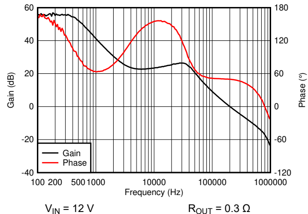
Figure 8-27. Bode Plot
