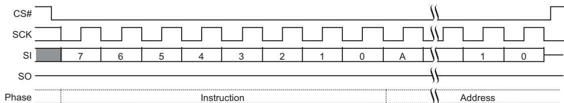
Figure 9.46 EES Command Sequence
