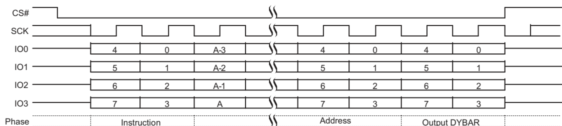
Figure 9.56 DYBRD QPI Mode Command Sequence
