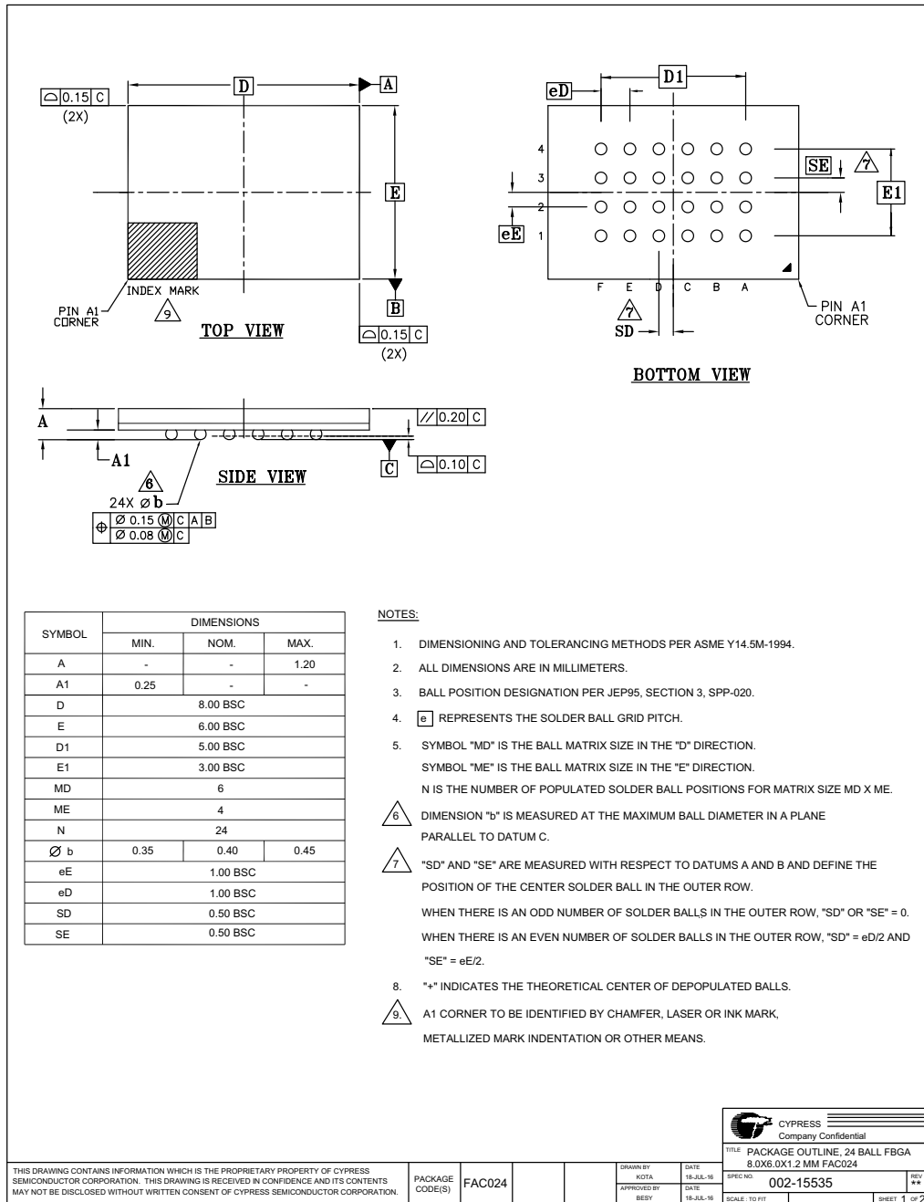
Figure 6.11 Ball Grid Array 24-Ball 6 x 8 mm (FAC024)
