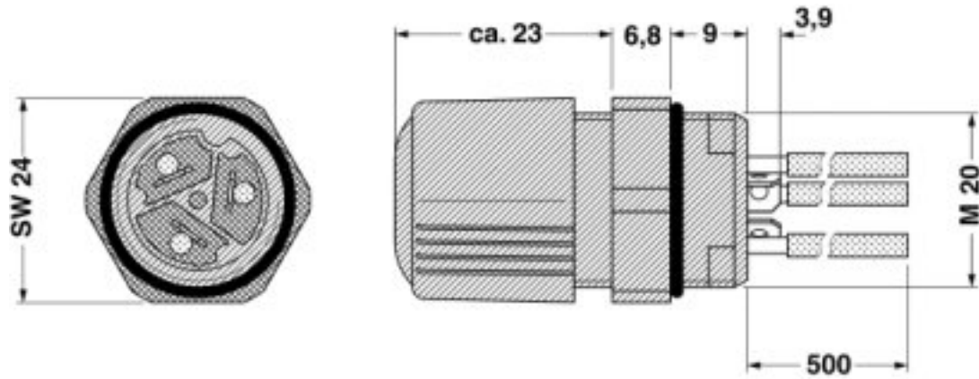
Dimensioned drawing
