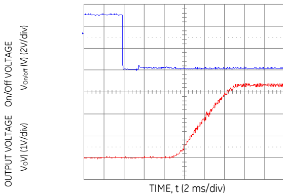
Figure 15. Typical Start-Up Using Remote On/Off with Low-ESR external capacitors (7x150uF Polymer) ( V_{in} = 5.0Vdc , V_o = 3.3Vdc , I_o = 6A , C_o = 1050\mu F ).
