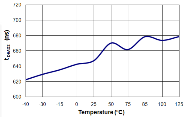
Figure 39. t_{\text{DEAD2}} ( R_{\text{RP}}=20 \text{ k} , 6 \mu\text{s} ) vs. T_{\text{A}}
