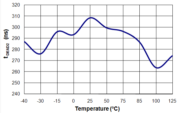
Figure 41. t_{\text{DEAD2}} ( R_{\text{RP}}=43 \text{ k} , 2.5 \mu\text{s} ) vs. T_{\text{A}}
