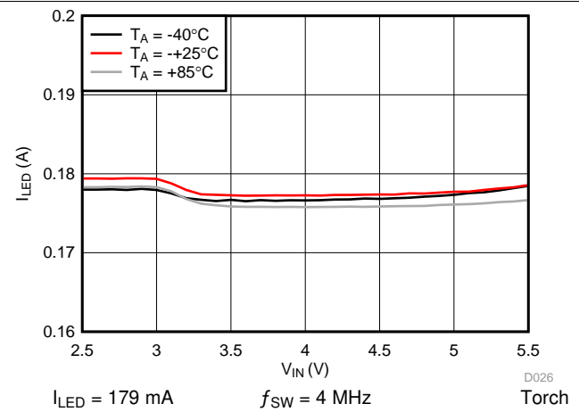
Figure 17. LED1 and LED2 Current vs Input Voltage
