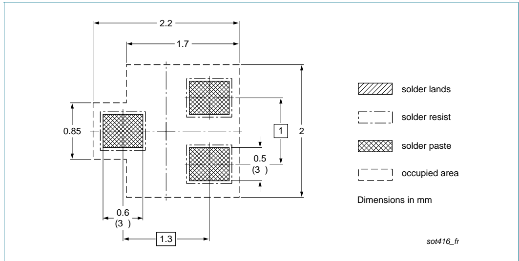
Fig 16. Reflow soldering footprint PDTA144EE (SOT416/SC-75)
