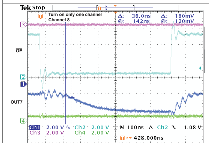
Figure 3. Response Time, \overline{OE} to OUT_7
