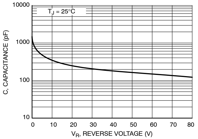
Figure 10. Capacitance
