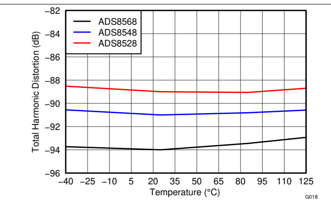
Figure 21. THD vs Temperature
