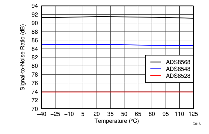
Figure 19. SNR vs Temperature
