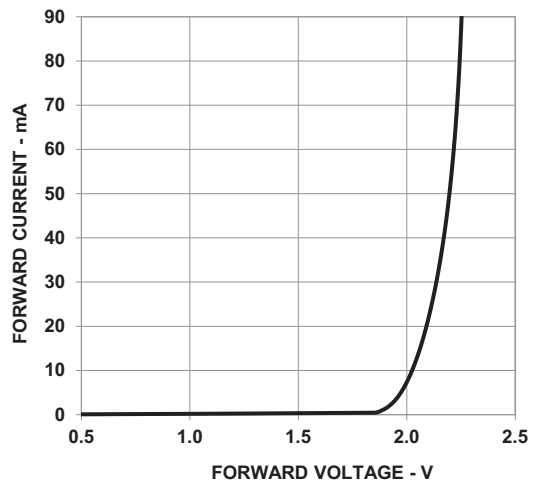
Figure 18: Forward Current vs. Forward Voltage
