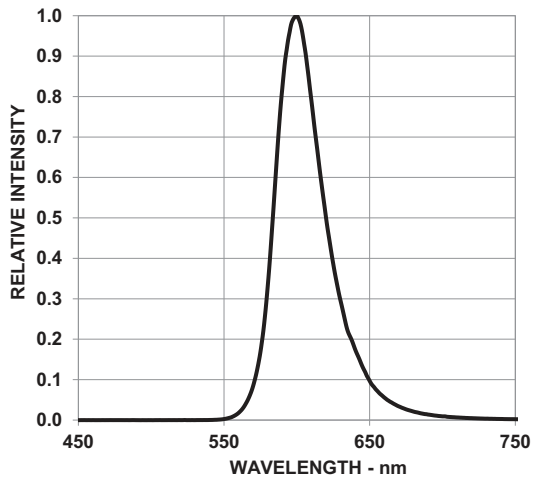
Figure 9: Relative Intensity vs. Wavelength
