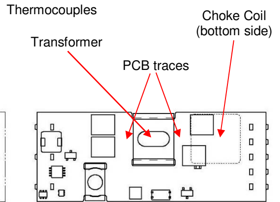
Fig. G: Location of thermocouples for thermal testing
