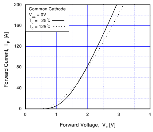
Fig 19. Forward Characteristics
