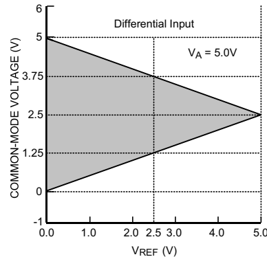
Figure 11. V_{CM} range for Differential Input operation
