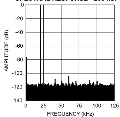
SPECTRAL RESPONSE - 250 KSPS
