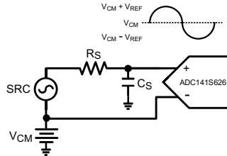
Figure 10. Single-Ended Input
