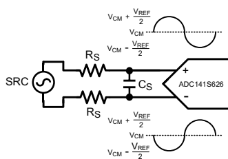
Figure 9. Differential Input
