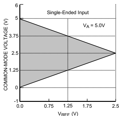
Figure 12. V_{CM} range for single-ended operation
