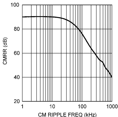
Figure 7. Analog Input CMRR vs. Frequency
