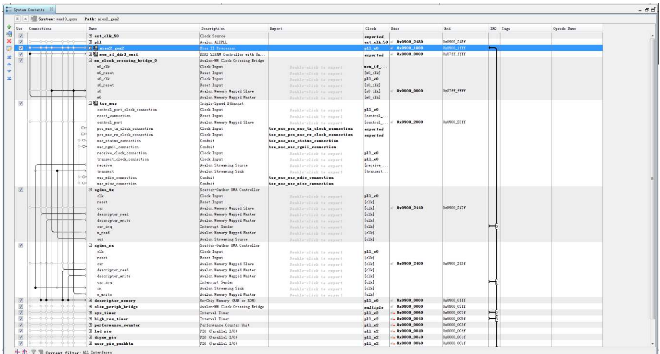
Figure 6-21 Qsys Builder
