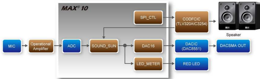
Figure 5-9 Block Diagram of the ADC/MIC/LED Demonstration
