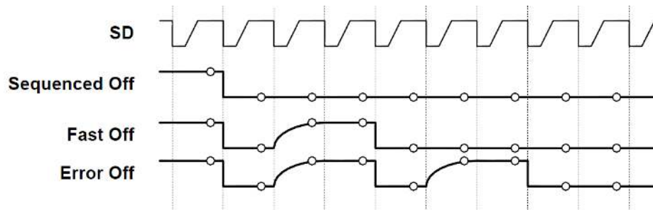
Figure 35. OK Severity Encoding Waveforms
