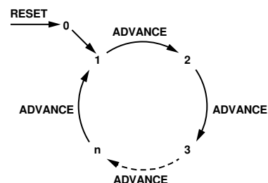
Figure 42. State Machine Position Loop
