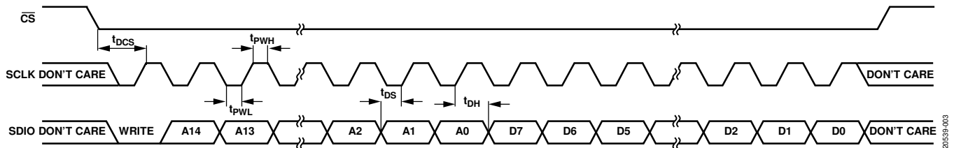
Figure 3. SPI Write Timing Diagram
