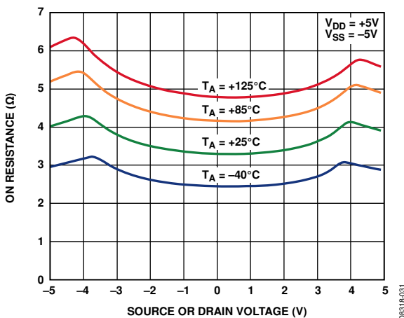
Figure 9. On Resistance vs. V_D (V_S) for Different Temperatures, \pm 5\text{ V} Dual Supply
