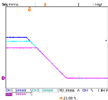
Figure 30. Tracking Turn-Off. Falling Slew Rate is Programmed at 0.5V/ms.
