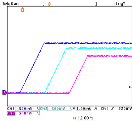
Figure 28 Two outputs delayed 5ms. All slew rates at 0.5V/ms
