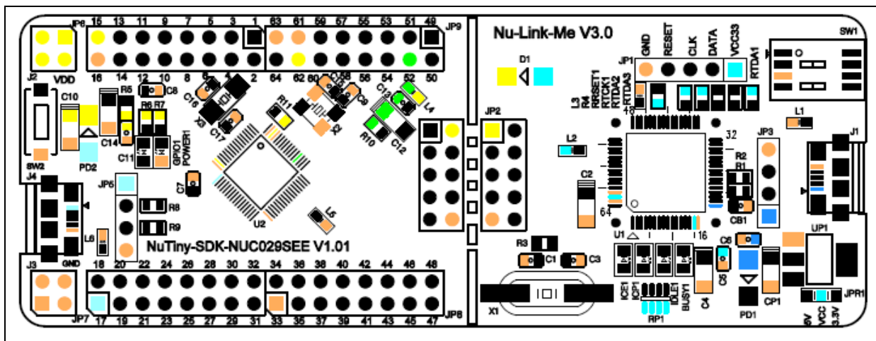
Figure 2-2 NuTiny-SDK-NUC029SEE PCB Placement
