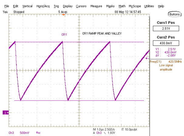
Figure 8 - Switching Frequency Tolerance
