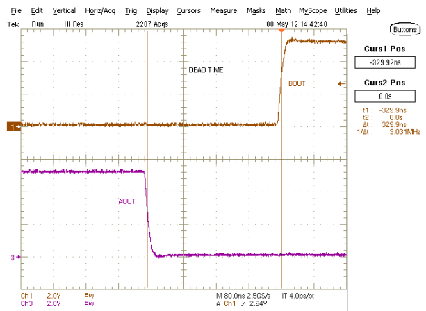
Figure 6 - Dead time between AOUT and BOUT
