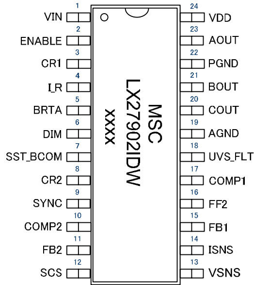
Figure 2 · Pinout
