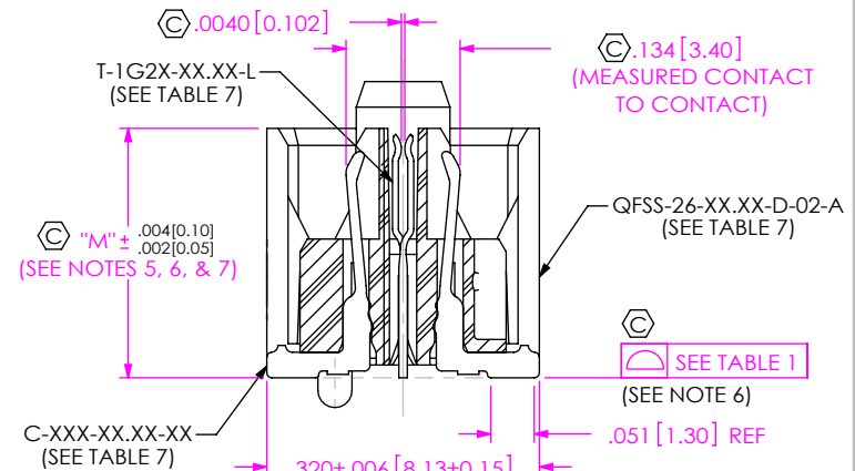
SECTION "A"-A" SCALE 5 : 1
