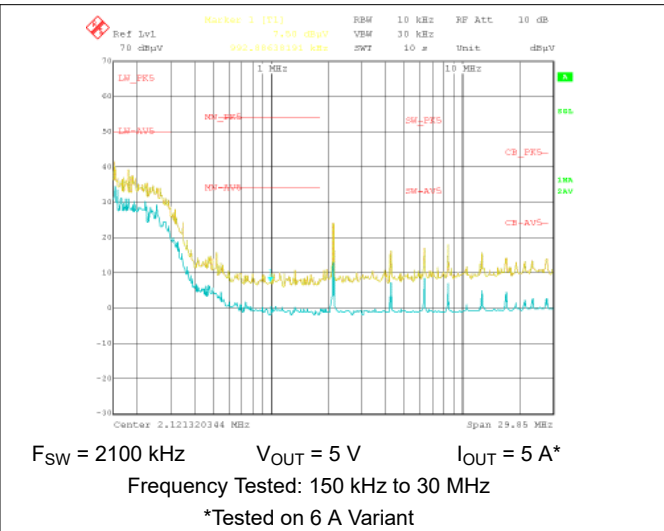
Figure 10-42. Conducted EMI versus CISPR25 Limits (Yellow: Peak Signal, Blue: Average Signal)
