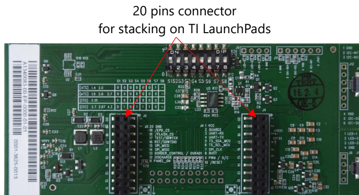
Figure 1-2 EPD Extension Board Gen2 (rear view)
