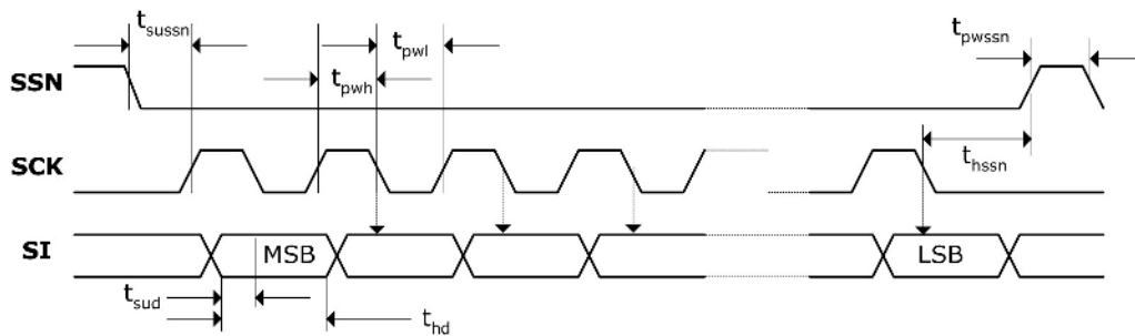
Figure 2-1: SPI Write
