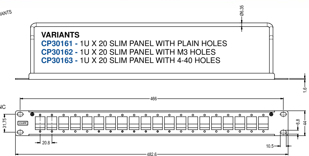
HOLE DETAIL (20x POSITIONS)
