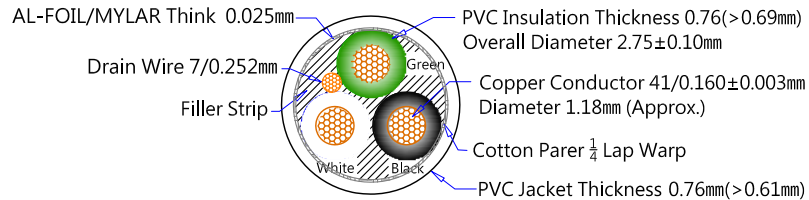
SJT 18AWGx3C Shielded(A+E) (Wire Cross-Section)
