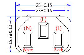
ME-302 (IEC 60320, C13) (Dimensions of Connector Face)
