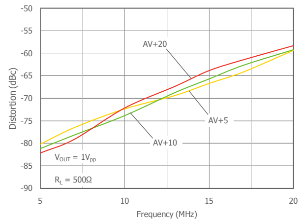
3rd Harmonic Distortion vs. Gain Freq at V_S = 5\text{V}
