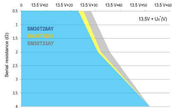
Figure 18. Load dump capability ( U_s^* = f(R_i) pulse 5b, U_s = 87\text{ V} , t_p = 150\text{ ms} )
