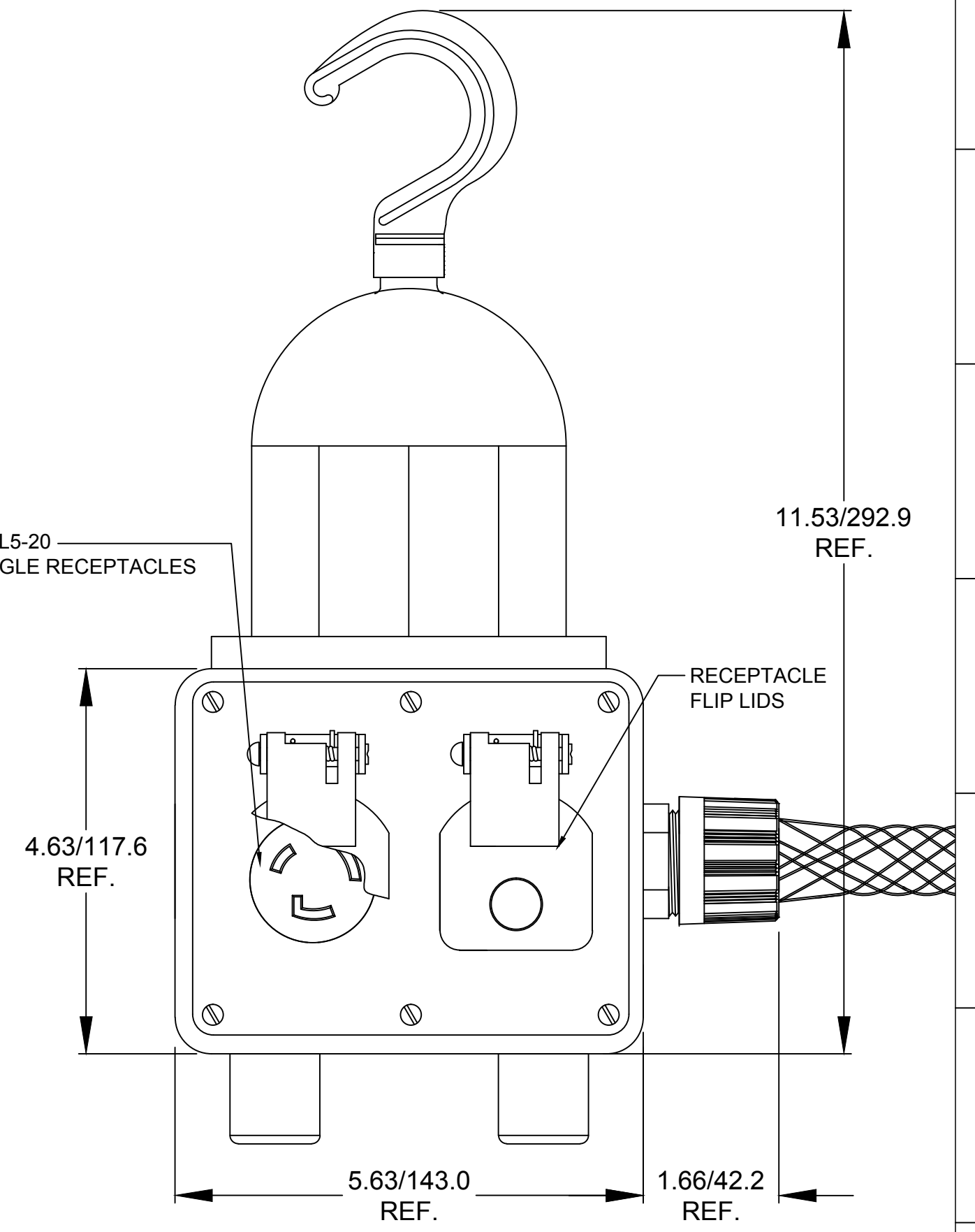
SIDE 2 (TWO NEMA L5-20 SINGLE RECPTACLES WITH FLIP LIDS)
