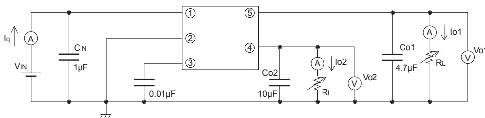
Fig.2 Standard measuring circuit of critical rate of ripple rejection
