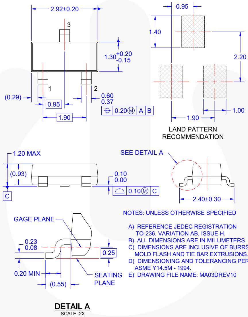
Figure 9. 3-LEAD, SOT23, JEDEC TO-236, LOW PROFILE (ACTIVE)
