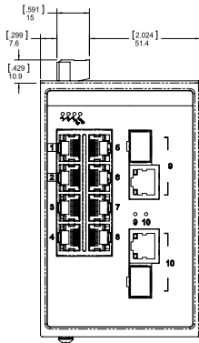
Model SEC410-2SFP-T faceplate detail
