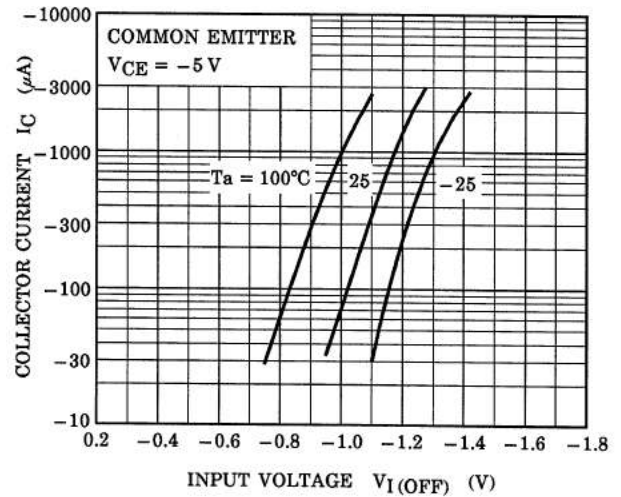
Fig. 10.4 RN2907 I_C - V_{I(OFF)}
