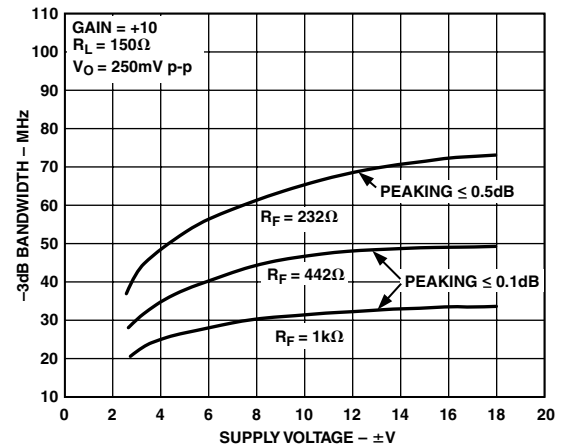
TPC 11. -3 dB Bandwidth vs. Supply Voltage, Gain = +10, R_L = 150 \Omega
