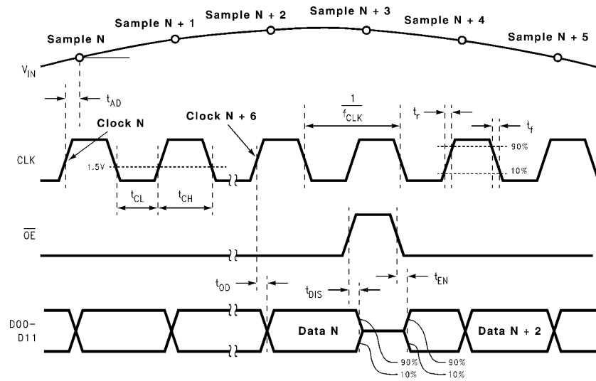
Figure 2. Output Timing
