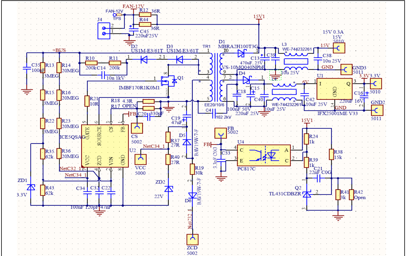
Figure 15 DC/DC power supply
