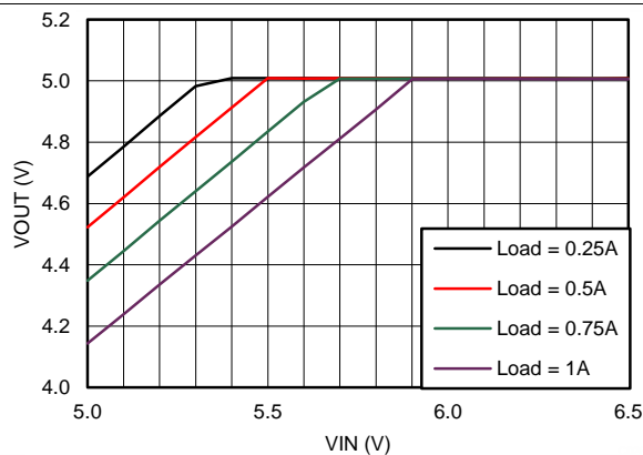
Figure 15. Dropout Curve
