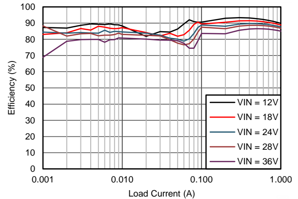
Figure 60. Efficiency
