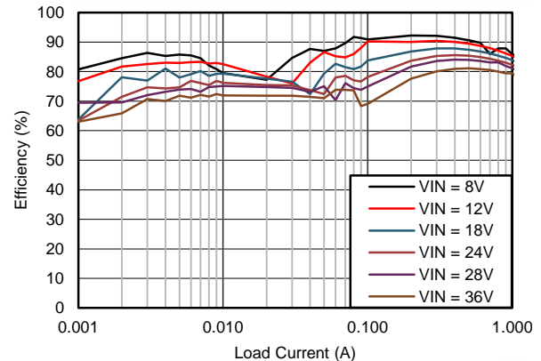
Figure 54. Efficiency
