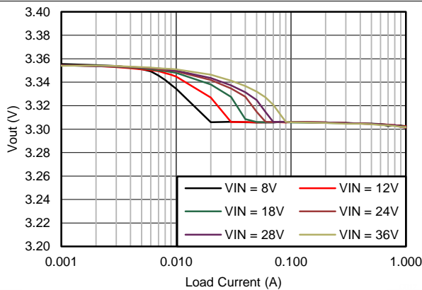
Figure 55. Output Voltage Regulation
